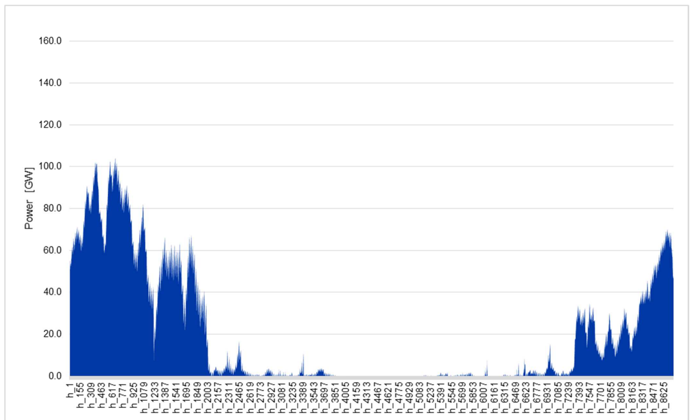
Figure 3 Hourly load profile of demand for electricity of heat pumps in the EU – Deep renovation
