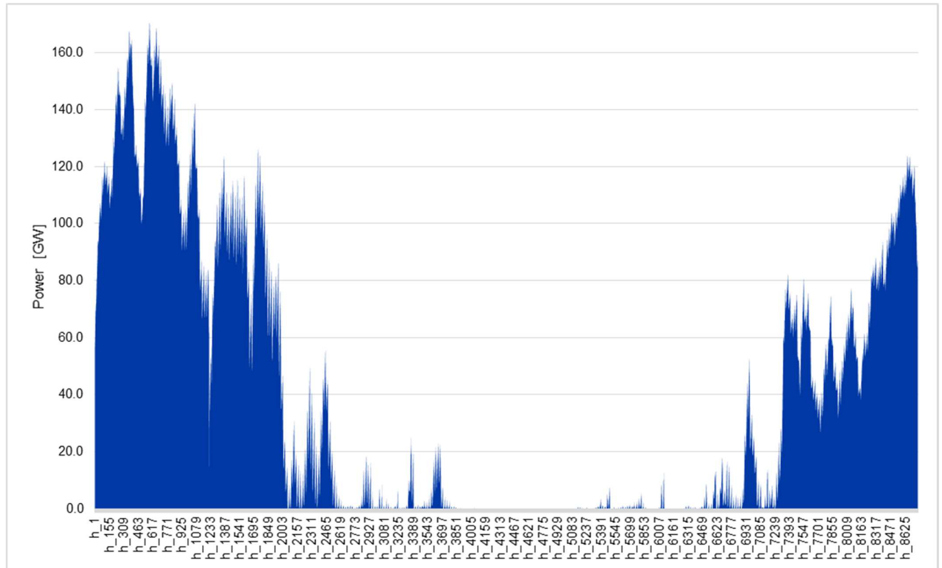
Figure 2 Hourly load profile of demand for electricity of heat pumps in the EU – Shallow renovation
