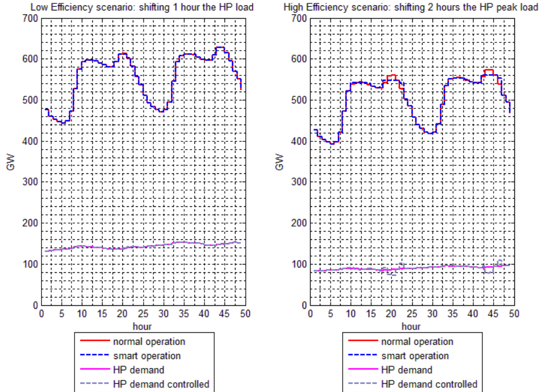
Figure 7: Daily load shape of the estimated EU electricity demand of buildings and the heat pump electricity consumption: Low Efficiency scenario with the option of shifting heat pump consumption by one hour (left) – High Efficiency scenario with the option of shifting heat pump consumption by two hours (right)
