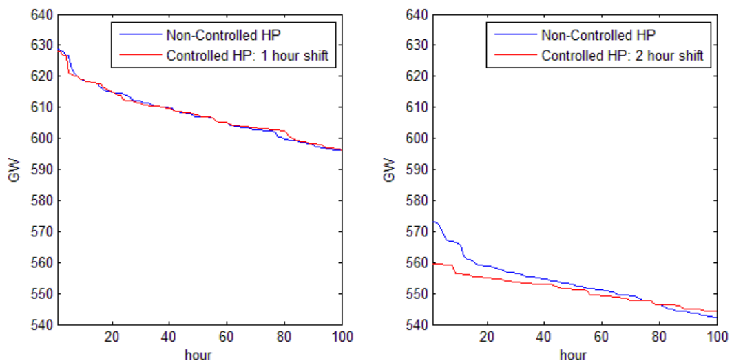
Figure 8 Load duration curve of each scenario showing the total impact of each heat demand flexibility option on the EU power system
