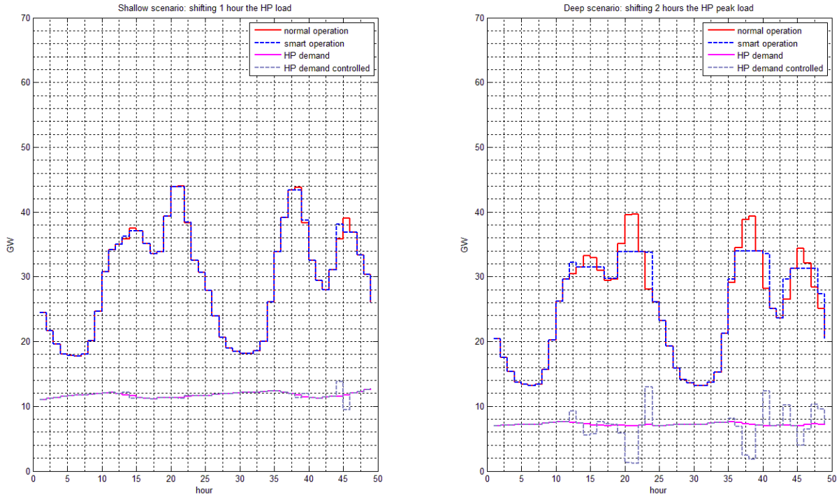
Figure 9 Daily load shape of the estimated residential buildings demand of Germany and the heat pump electricity consumption: Low Efficiency scenario with the option of shifting heat pump consumption by one hour (left) – High Efficiency scenario with the option of shifting heat pump consumption by two hours (right)
