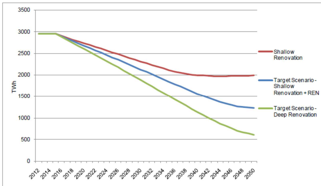
Figure 1 Final energy for space heating EU27 [TWh] without new buildings [3]
