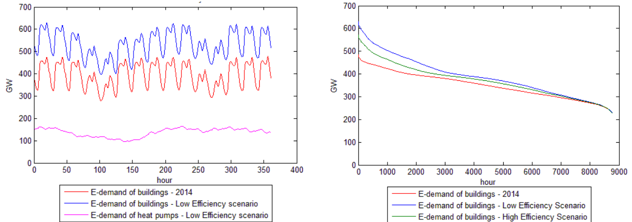
Figure 6: Increase of heat demand from buildings to the EU system load: Time series for 2 weeks in January showing the respective patterns (left) and load duration curves showing the total impact (right)
